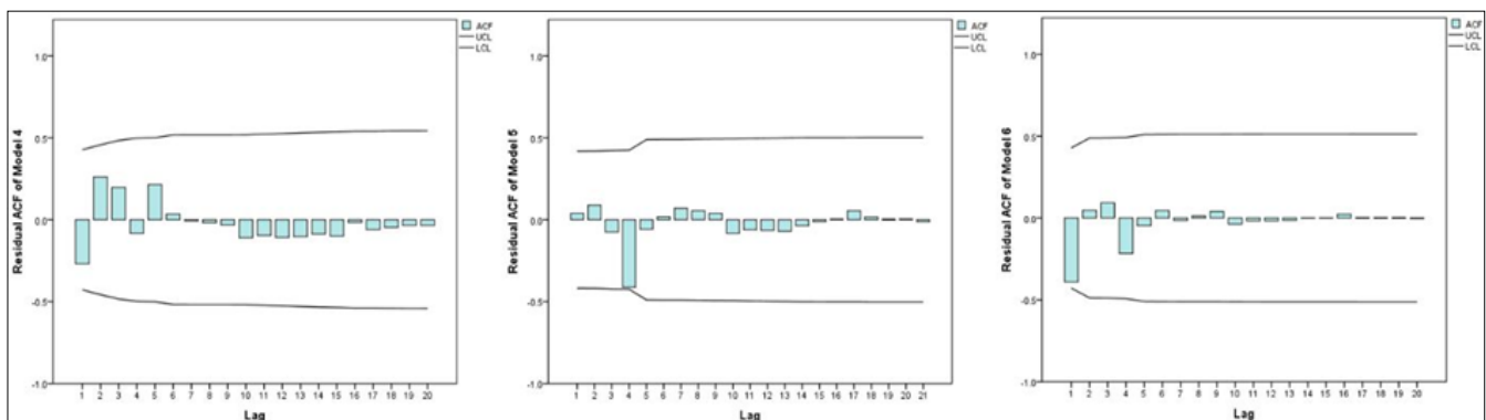
Figure 2. Residual ACF of six time series models of cumulative confirmed cases in mainland China.
