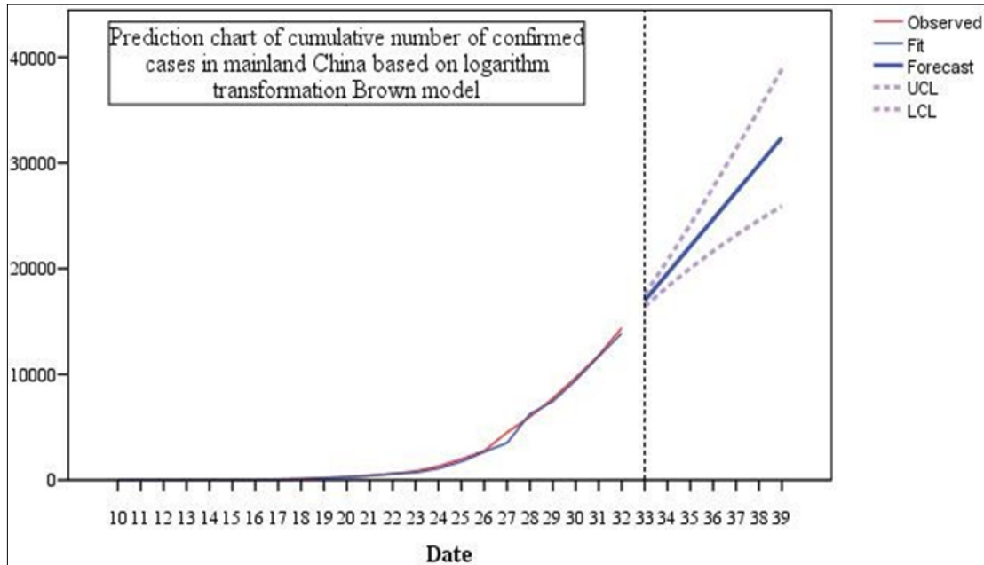
Figure 3. Prediction chart of cumulative number of confirmed cases in mainland China based on logarithm transformation Brown model.
