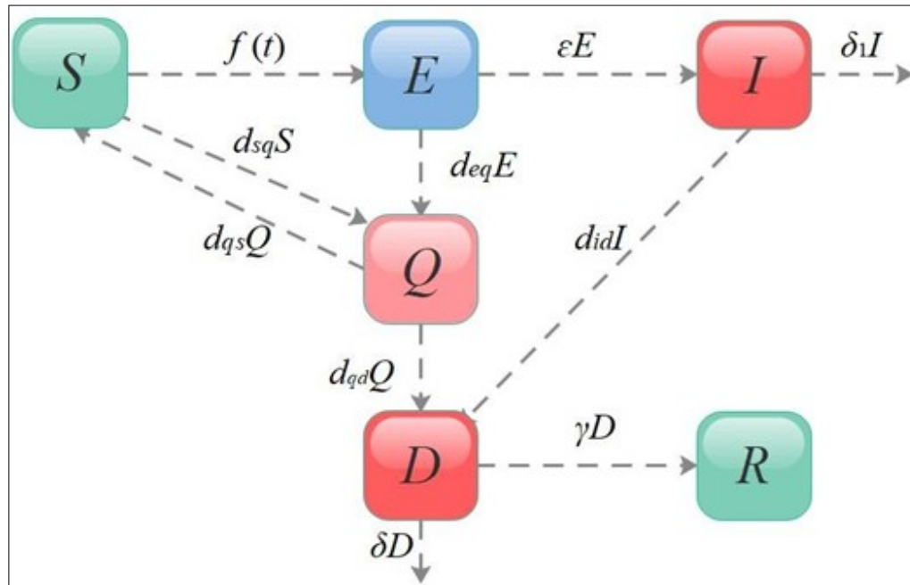
Figure 1. Warehouse transfer diagram of SEIQDR Model.
